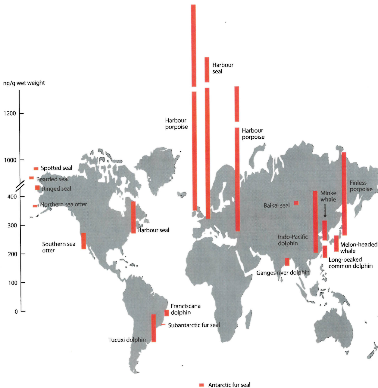
Figure 18. EDCs are found in wildlife worldwide. This figure shows concentrations (in ng/g wet weight) of per-fluorooctane sulfonate, also known as PFOS, in liver of marine mammals (modified from Houde et al., 2011).
