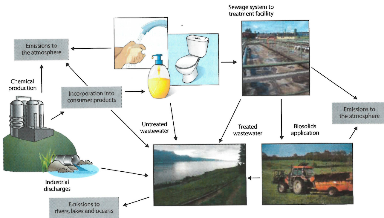
Figure 16. EDCs find their way into the environment via point and diffuse sources, as illustrated here.
